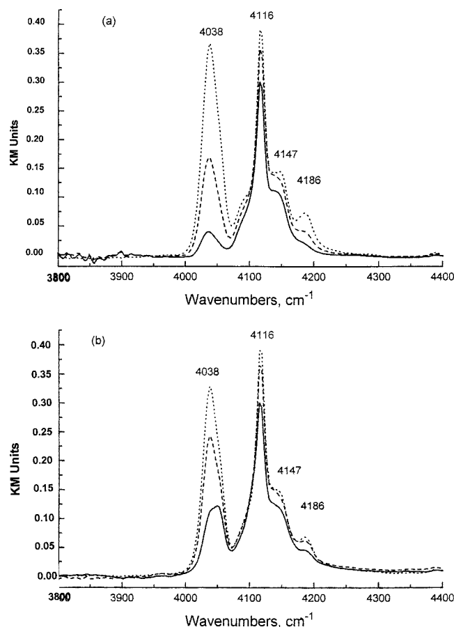
Figure 3. (a) DRIFT spectra of molecular hydrogen adsorbed at 77 K and an equilibrium pressure of 13.3 kPa on ZnY zeolite evacuated at 570 (—), 673 (---) and 770 (···). (b) DRIFT spectra of molecular hydrogen adsorbed at 77 K and an equilibrium pressure of 13.3 kPa on sulfided ZnY zeolite evacuated at 570 (—), 670 (---) and 770 K (···).
